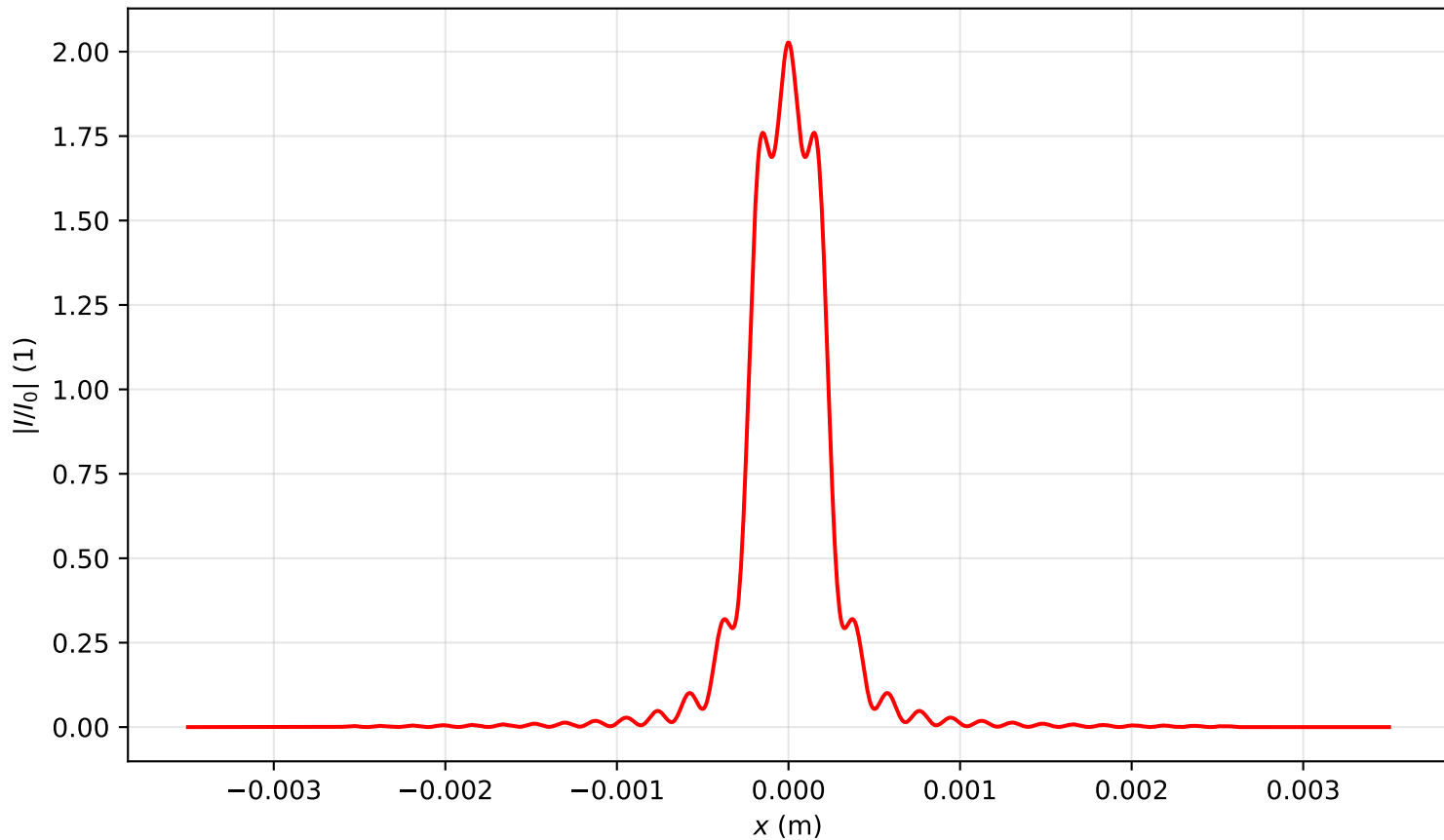
Intensity profile I(x, y = 0, z = 0.159)/I_0 , P_{in}=2.0P_{cr} , artificial time
